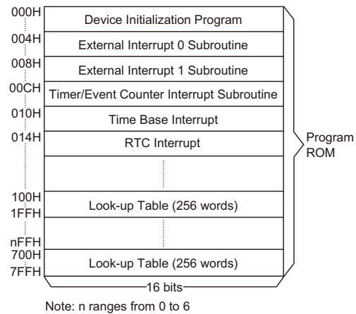
Program Memory
