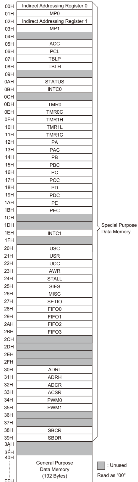
RAM Mapping
