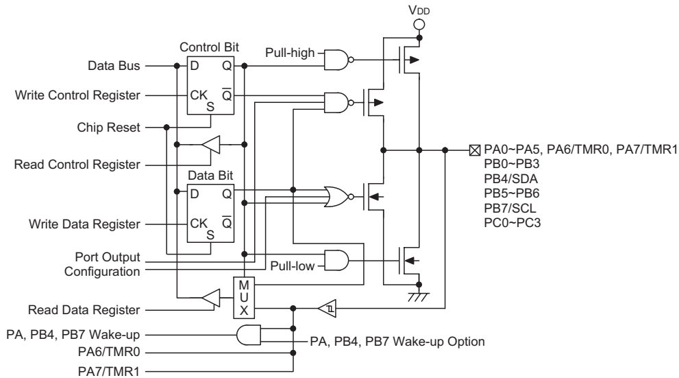
Input/Output Ports
