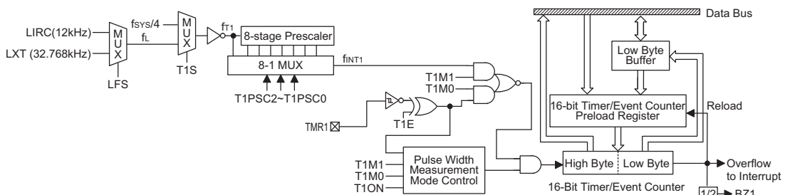
Timer/Event Counter 1
