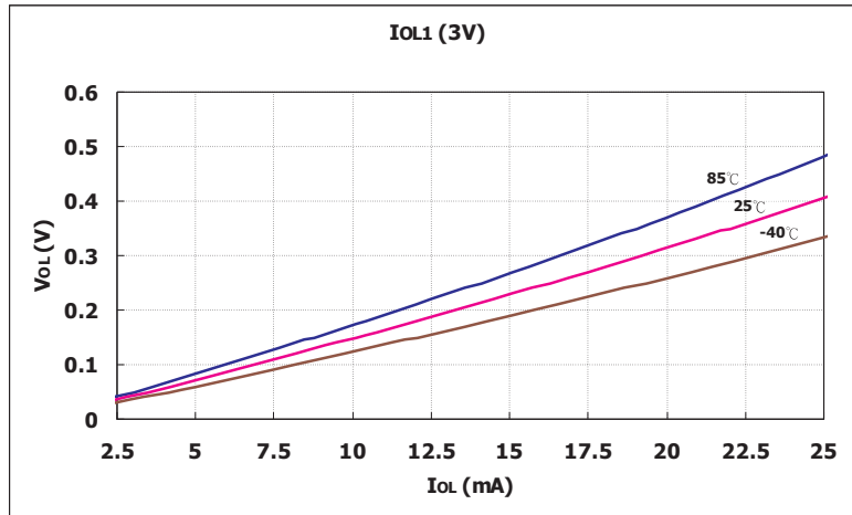
V_{OL} vs. I_{OL1} Over Temperature ( V_{DD}=3.0V )
