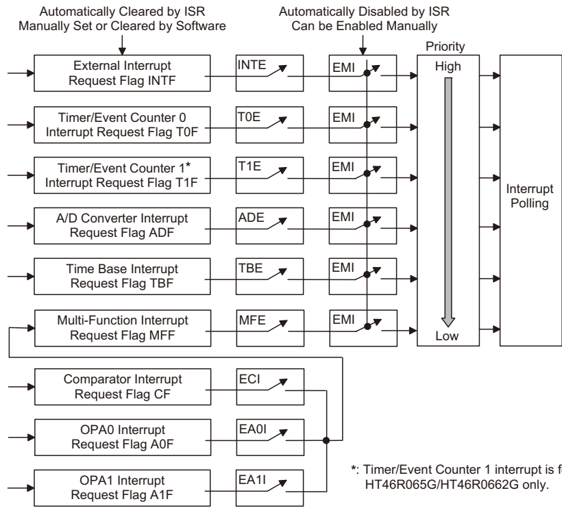
Interrupt Scheme
