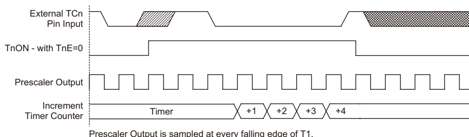
Pulse Width Capture Mode Timing Chart (TnE=0)
