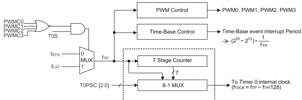
Clock Structure for Timer/PWM/Time Base
