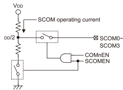
SCOM Circuit
