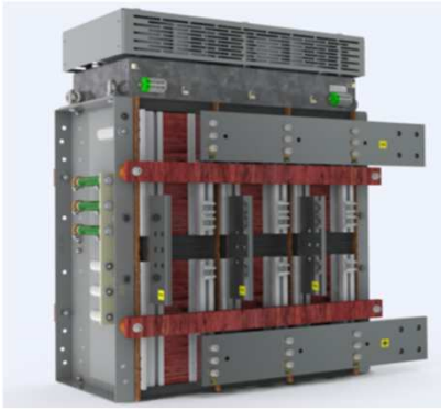
Thyristor/Diode Presspack stack
