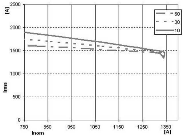
Fig. 2 Maximum overload current, T_{amb} = 50\text{ }^{\circ}\text{C}
