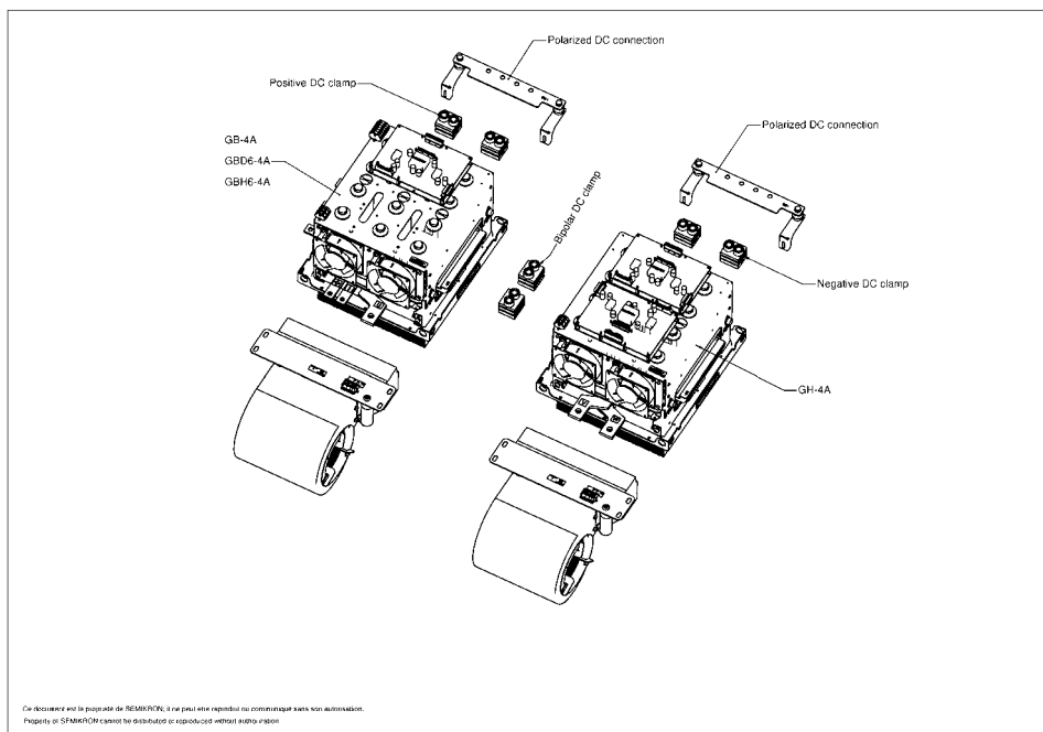
3D view of the SEMIKUBE Size '2'
