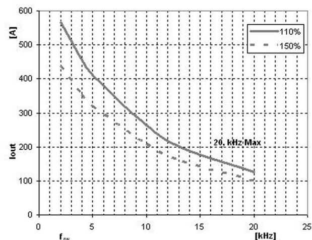
Fig. 4 Max. permanent inverter curr. vs. f_{sw} , T_{amb}=50\text{ }^{\circ}\text{C}
