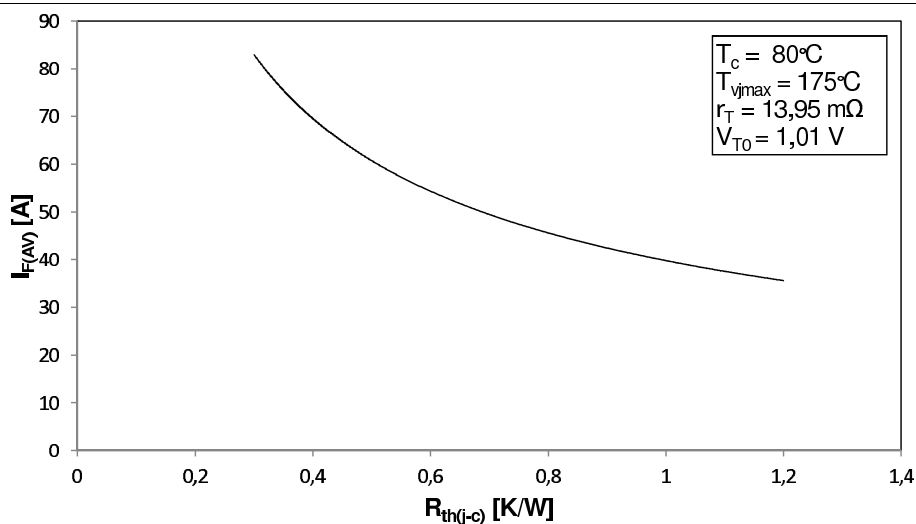
Fig. 1: Rated current vs. thermal resistance
