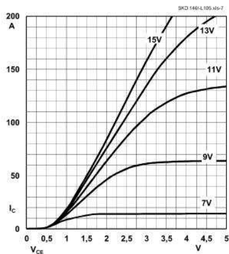
Fig. 7 Output IGBT characteristic I_C = f(V_{CE}) , T_j = 125^\circ\text{C}
