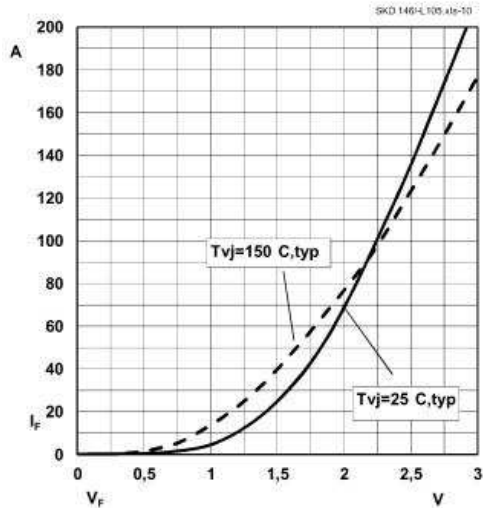
Fig. 10 Diode forward characteristic
