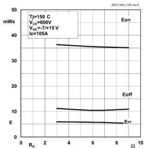
Fig. 9 Turn-on/-off energy =f(R_g)
