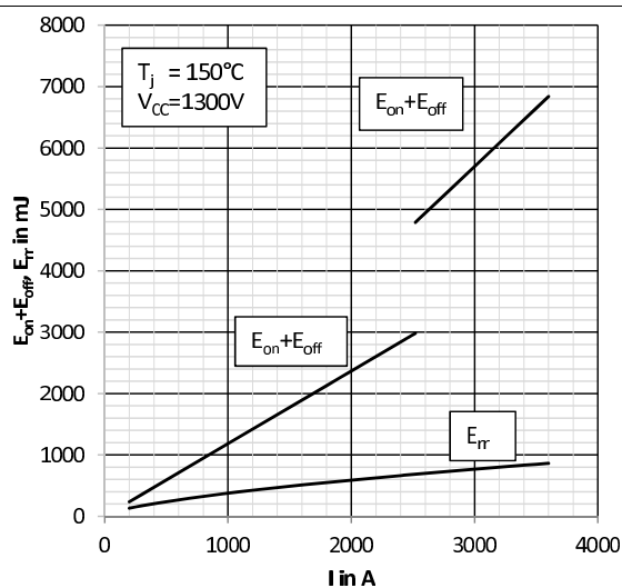
Fig. 4: Typical switching energy E = f(I_C)
