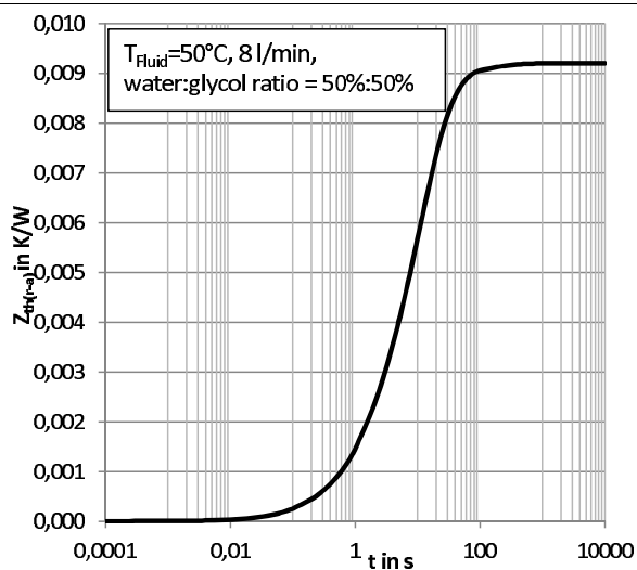
Fig. 7: Transient thermal impedance Z_{\text{th}}(\text{r-a})
