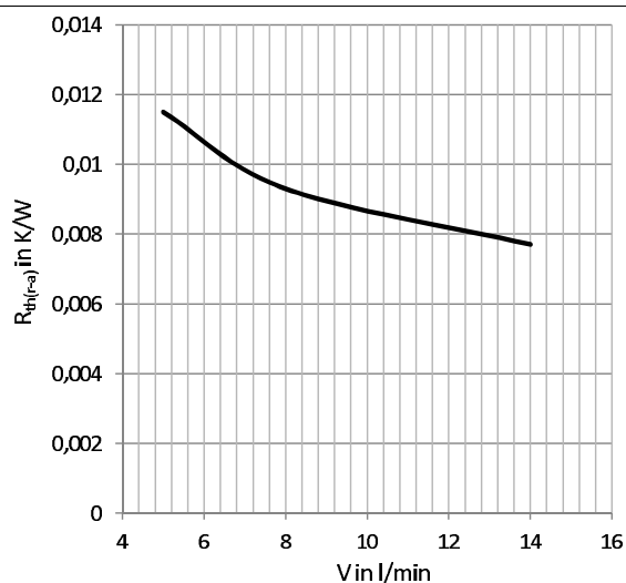
Fig. 9: Thermal resistance R_{\text{th}}(\text{r-a}) versus flow rate V
