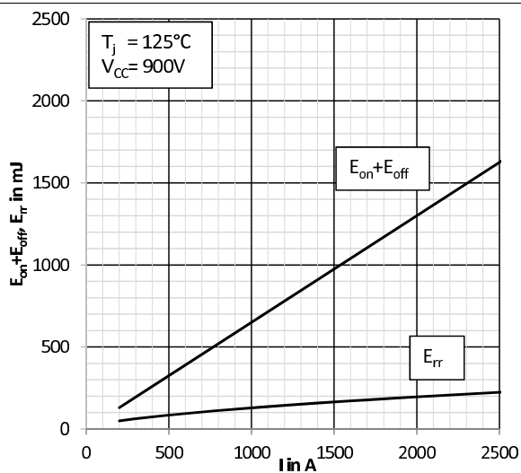
Fig. 3: Typical energy losses E = f(I_C, V_{CC})
