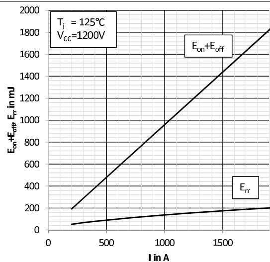
Fig. 4: Typical energy losses E = f(I_C, V_{CC})
