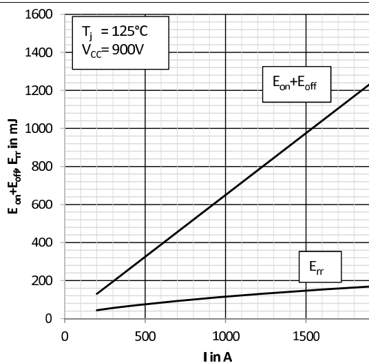
Fig. 3: Typical energy losses E = f(I_C, V_{CC})
