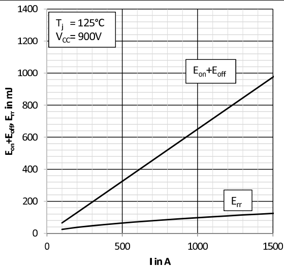
Fig. 3: Typical energy losses E = f(I_C, V_{CC})
