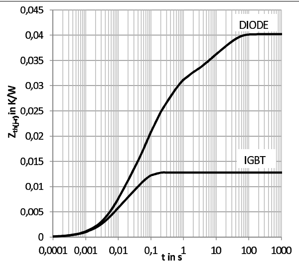
Fig. 6: Transient thermal impedance Z_{th}(j-\tau)
