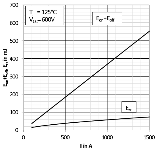
Fig. 3: Typical energy losses E = f(I_C, V_{CC})
