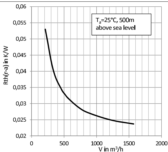
Fig. 9: Thermal resistance R_{th}(r-a) versus flow rate V
