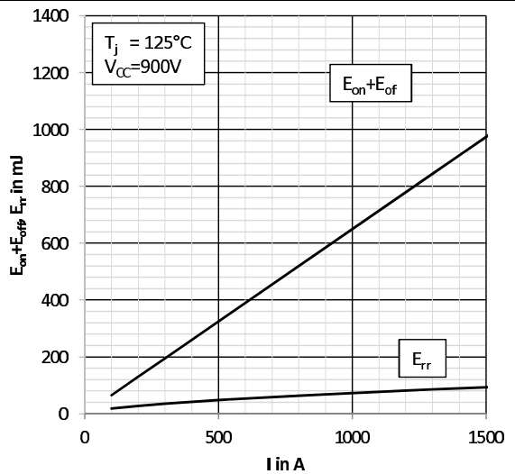
Fig. 4: Typical energy losses E = f(I_C, V_{CC})
