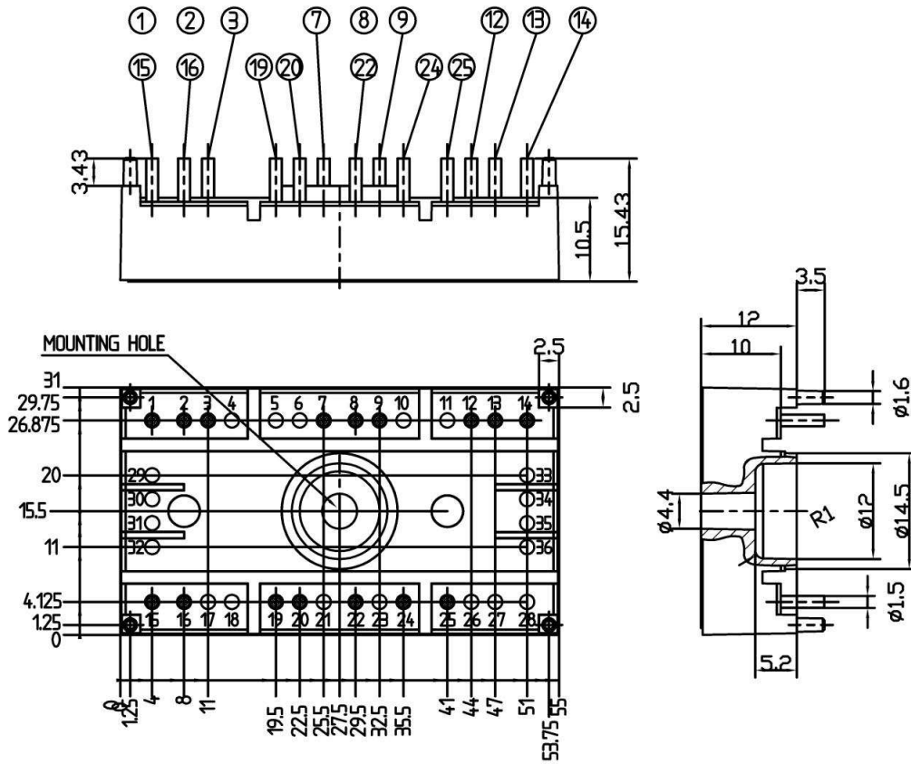
Case T16 (Suggested hole diameter, in the PCB, for solder pins and plastic mounting pins: 2mm)
