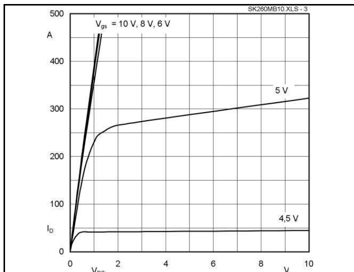
Fig. 3 Output characteristic, t_p = 80\text{ }\mu\text{s} , T_j = 25\text{ }^\circ\text{C}
