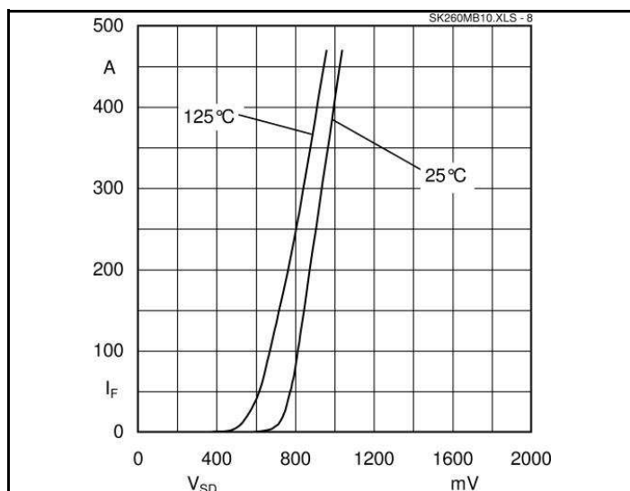
Fig. 8 Diode forward characteristic, t_p = 80\text{ }\mu\text{s}
