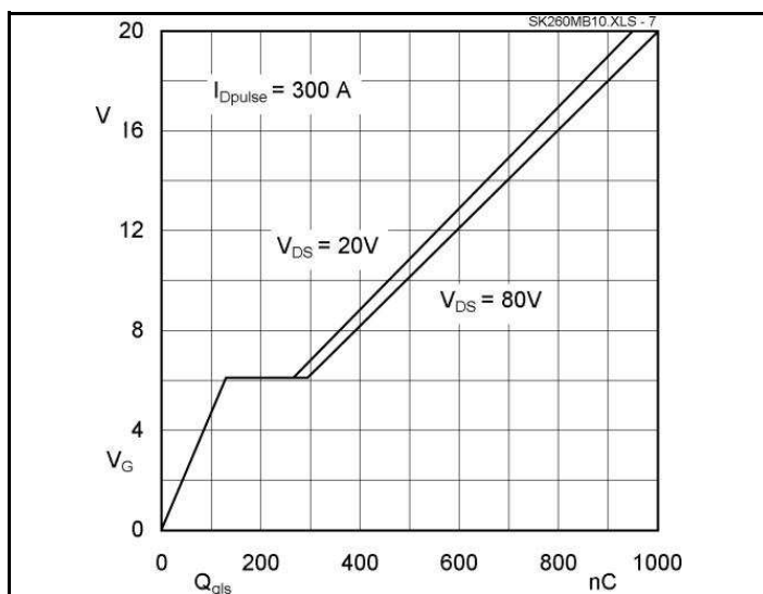
Fig. 7 Gate charge characteristic, I_{Dp} = 300\text{ A}
