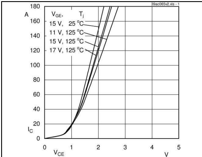
Fig. 1 Output characteristic
