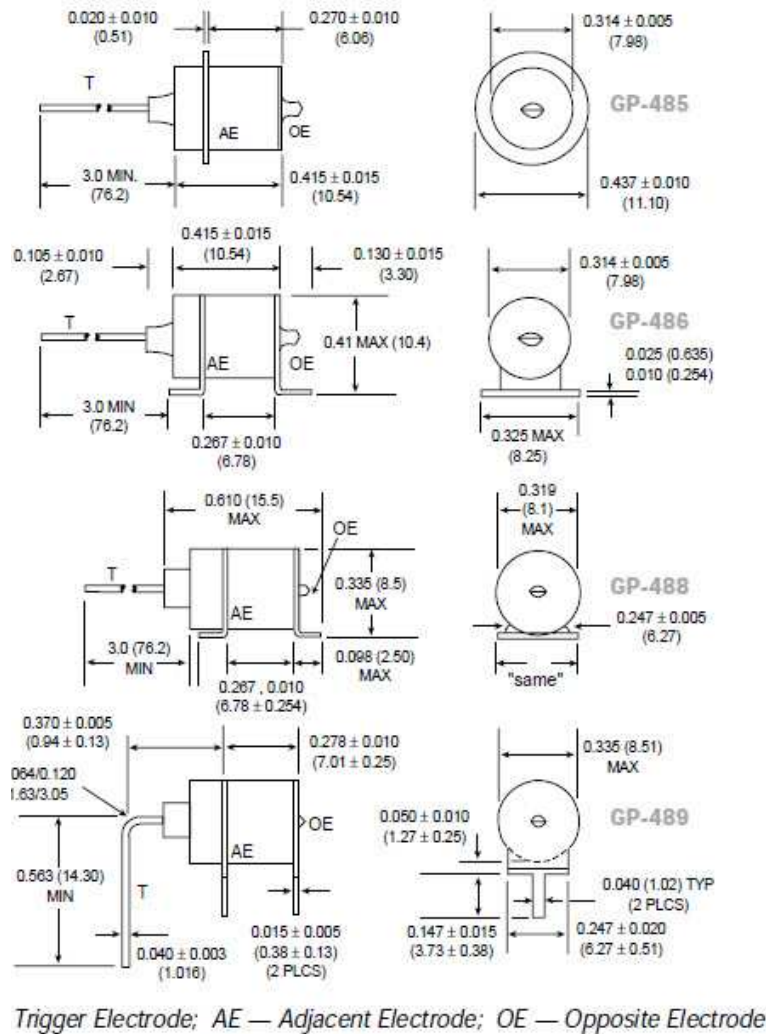
FIGURE 4 Mechanical Specifications
