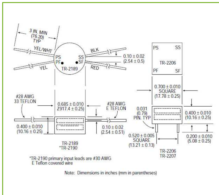
FIGURE 8 Mechanical Specifications
