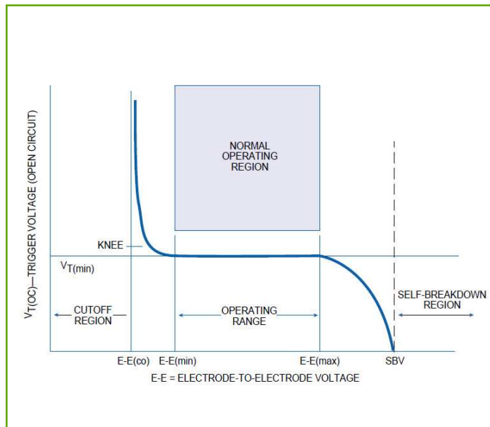
FIGURE 3 Transfer Characteristics
