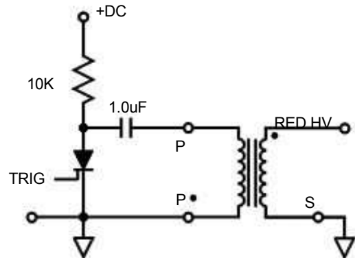
TYPICAL CIRCUIT
