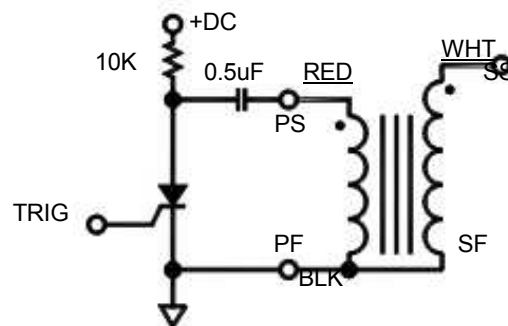
TYPICAL CIRCUIT
