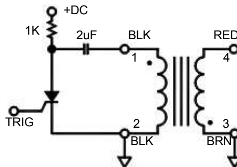
TYPICAL CIRCUIT
