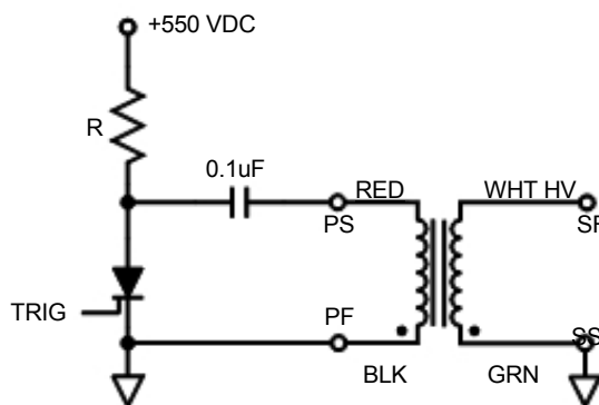
TYPICAL CIRCUIT
