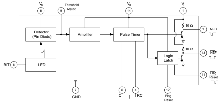
Logic Diagram
