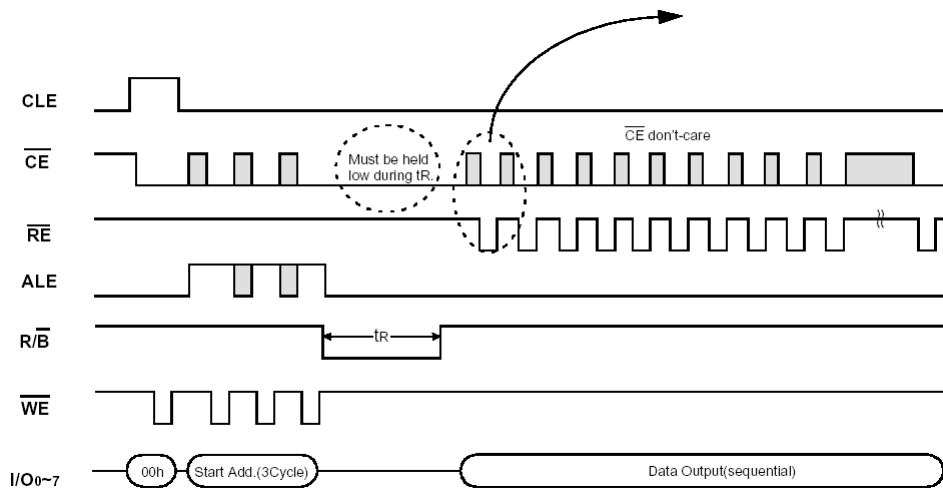
FIGURE 9. READ OPERATION WITH CE DON'T CARE
