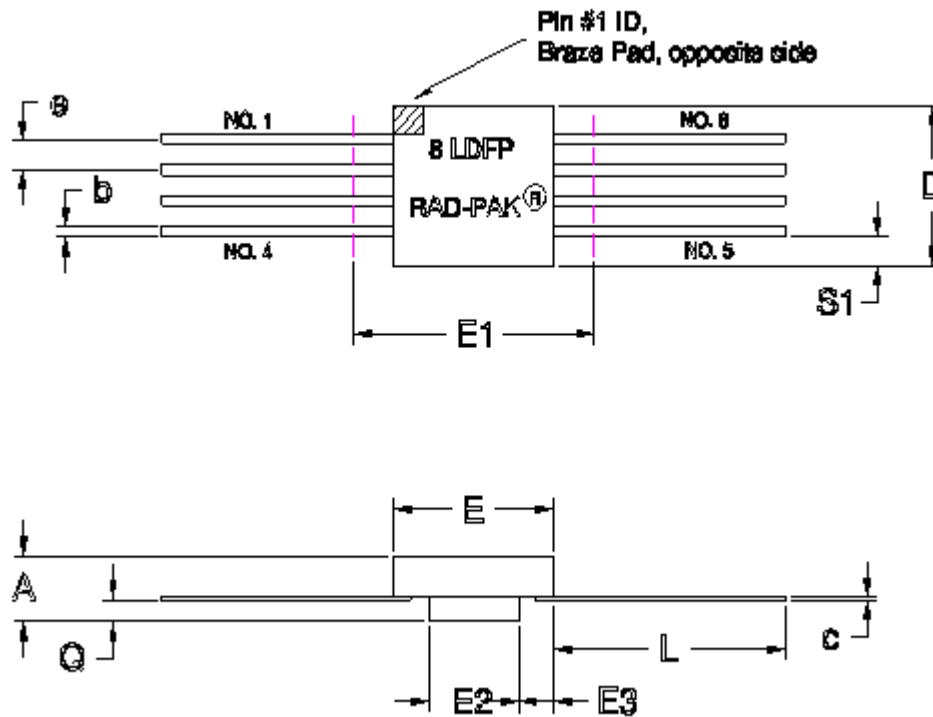
8-PIN RAD-PAK® FLAT PACKAGE
