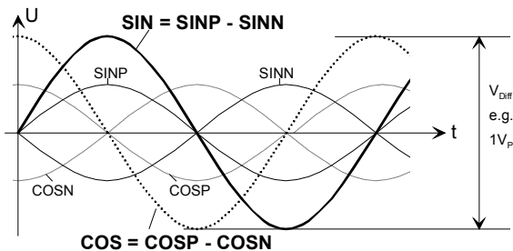
Figure 2 Input Signals Instrumentation Amplifier
