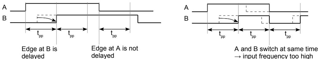
Figure 7 Minimum Edge Distance
