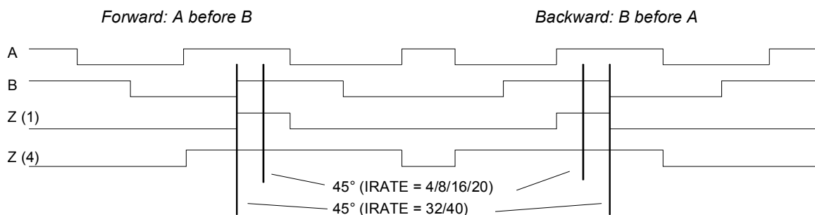
Figure 5 Output Signals Interpolation
