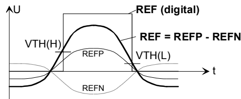
Figure 3 Reference Point Comparator
