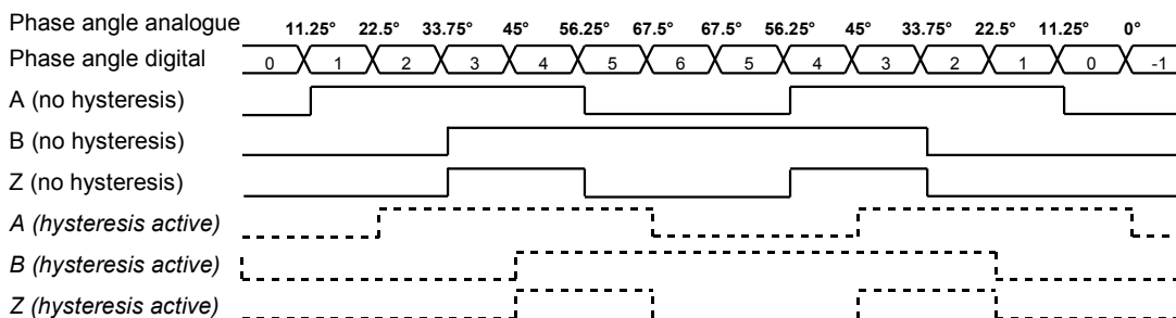
Figure 6 Digital Hysteresis
