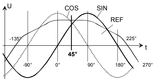
Figure 4 Input Signals Interpolation
