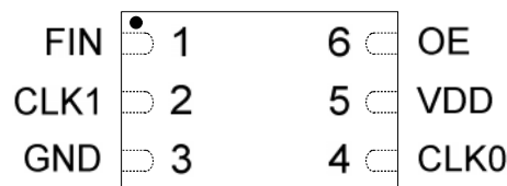
DFN-6L (2.0 x 1.3 x 0.6mm)
