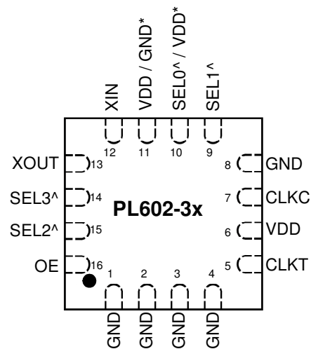
QFN-16L
