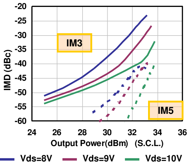
IMD vs. Output Power by Drain Voltage
