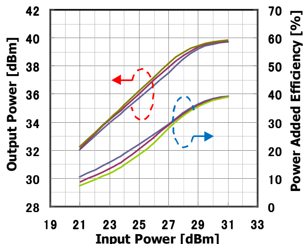
Input Power vs. Output Power, Power Added Efficiency by Quiescent Drain Current V_{DS}=10V @7.5GHz
