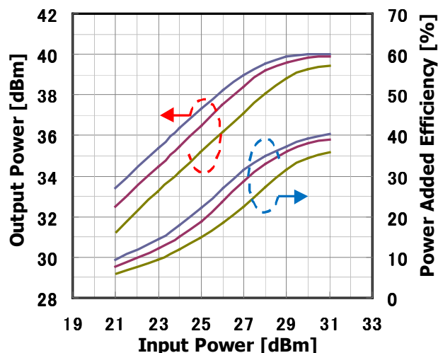
Input Power vs. Output Power, Power Added Efficiency by Temperature V_{DS}=10V I_{DS(DC)}=2200mA @7.5GHz
