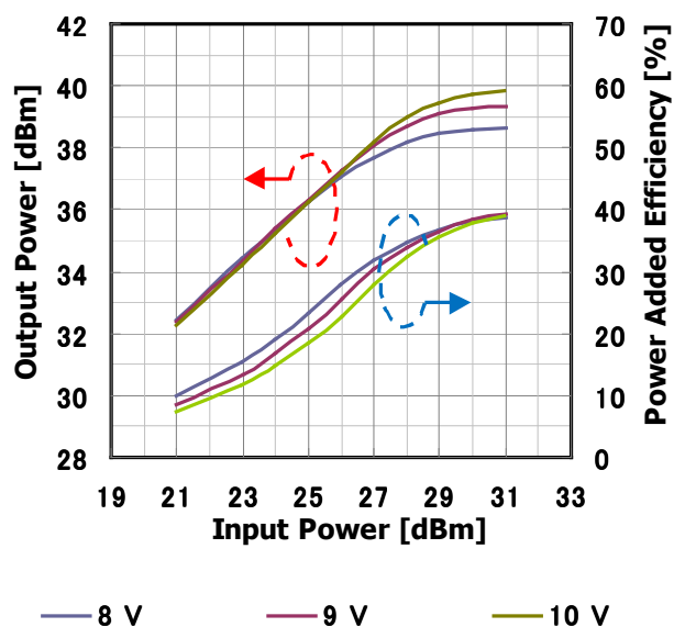
Input Power vs. Output Power, Power Added Efficiency by Drain Voltage I_{DS(DC)} = 2200\text{mA} @ 7.5GHz
