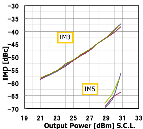
IMD Performance vs. Output Power by Drain Voltage I_{DS(DC)} = 2200\text{mA} @ 7.1GHz
