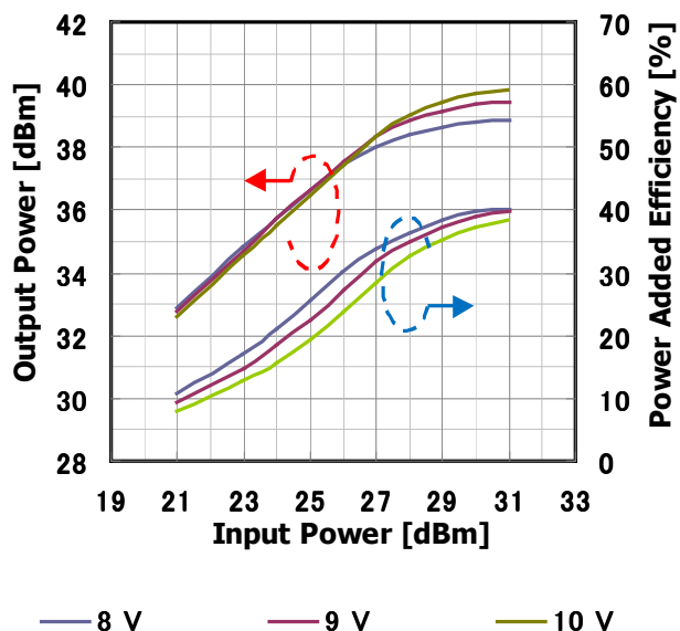
Input Power vs. Output Power, Power Added Efficiency by Drain Voltage I_{DS(DC)} = 2200\text{mA} @ 7.1GHz
