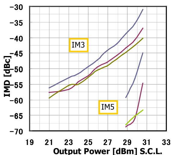
IMD Performance vs. Output Power by Drain Voltage I_{DS(DC)} = 2200\text{mA} @ 7.9GHz
