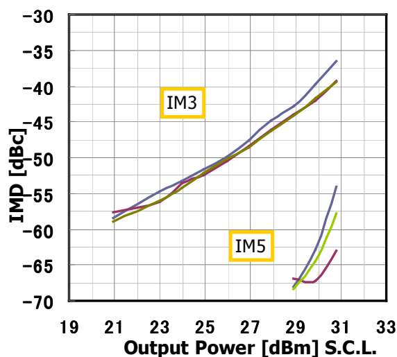
IMD Performance vs. Output Power by Drain Voltage I_{DS(DC)} = 2200\text{mA} @ 7.5GHz
