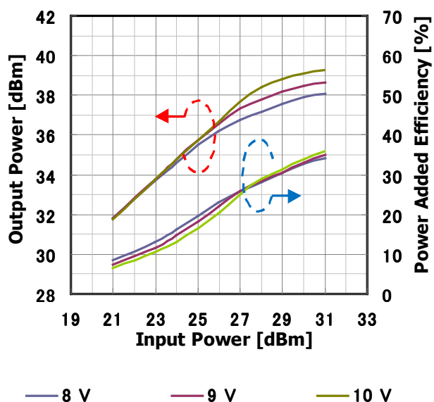
Input Power vs. Output Power, Power Added Efficiency by Drain Voltage I_{DS(DC)} = 2200\text{mA} @ 7.9GHz
