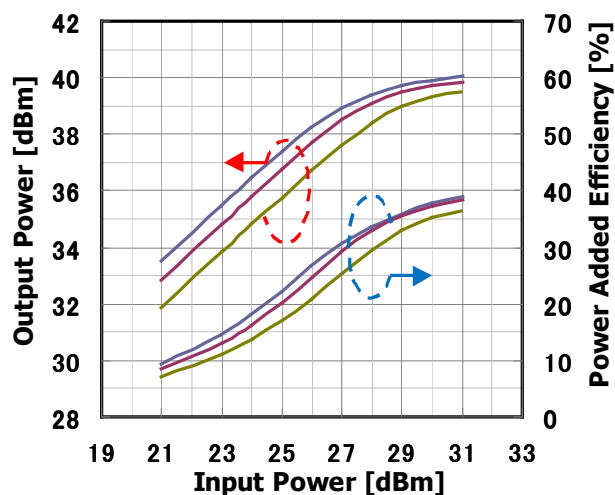
Input Power vs. Output Power, Power Added Efficiency by Temperature V_{DS}=10V I_{DS(DC)}=2200mA @7.1GHz
