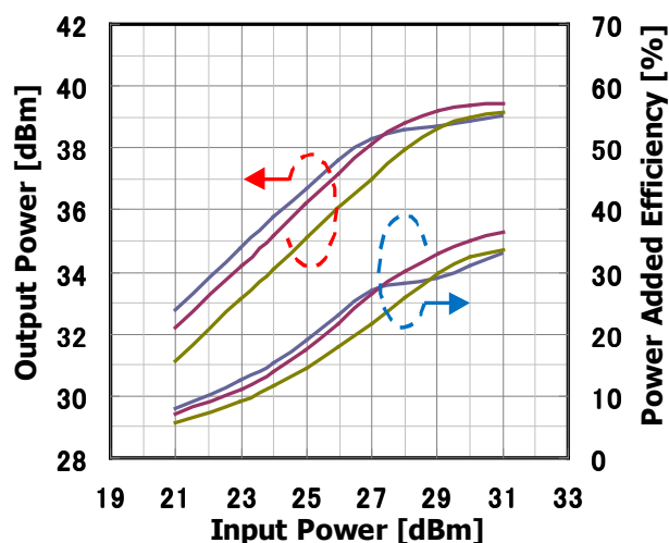
Input Power vs. Output Power, Power Added Efficiency by Temperature V_{DS}=10V I_{DS(DC)}=2200mA @7.9GHz
