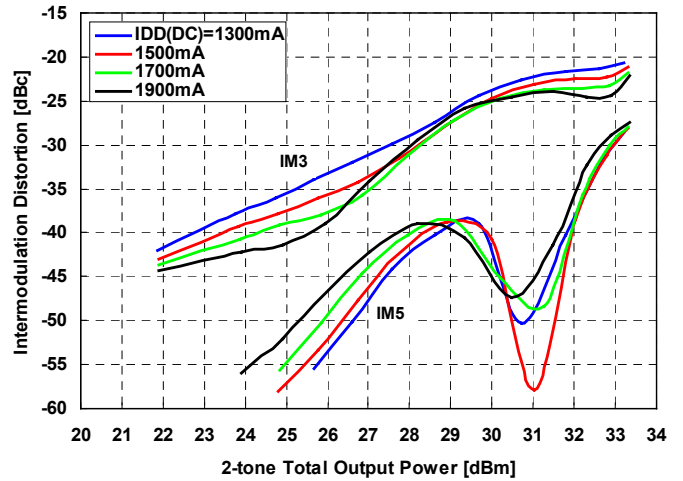
IMD vs. Output Power by Drain Current
