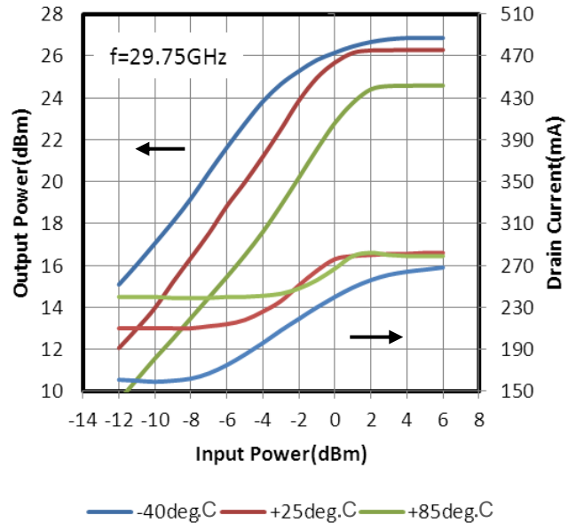
OUTPUT POWER, DRAIN CURRENT vs. INPUT POWER by Drain Current Frequency=29.75GHz
