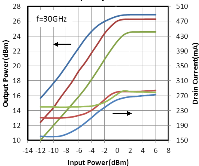
OUTPUT POWER, DRAIN CURRENT vs. INPUT POWER by Temperature Frequency=30.0GHz
