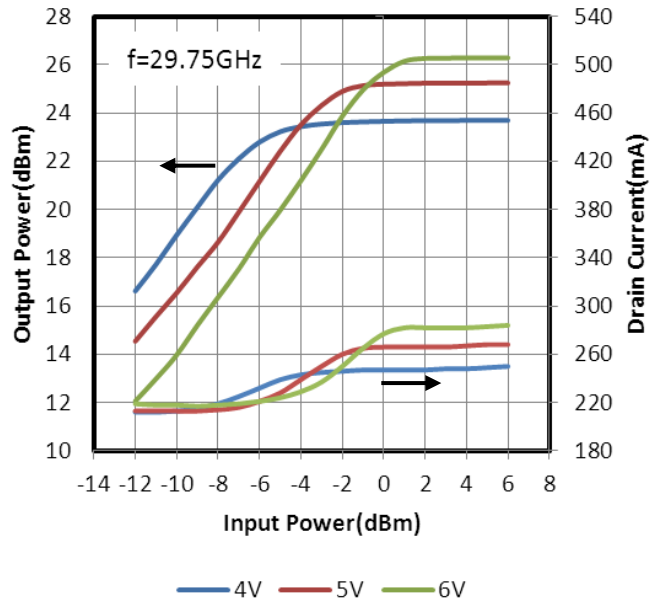
OUTPUT POWER, DRAIN CURRENT vs. INPUT POWER by Drain Voltage Frequency=29.75GHz
