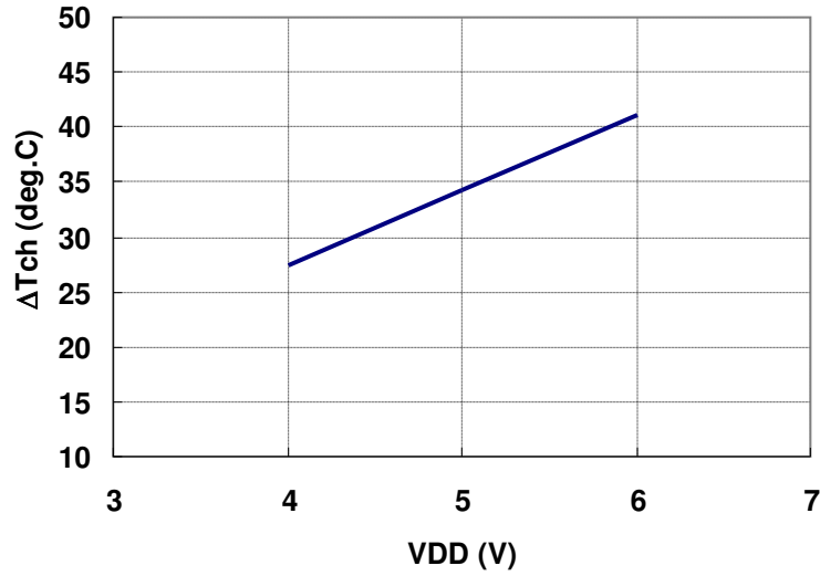
\Delta T_{ch} vs. Drain Voltage (Reference)
