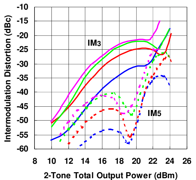
IMD Performance vs. Total Output Power @ V_{DD}=6V , I_{DD(DC)}=250mA \Delta f=+10MHz , 2-Tone test
