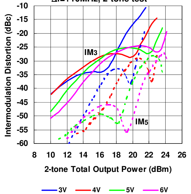
IMD Performance vs. Total Output Power by Drain Voltage
