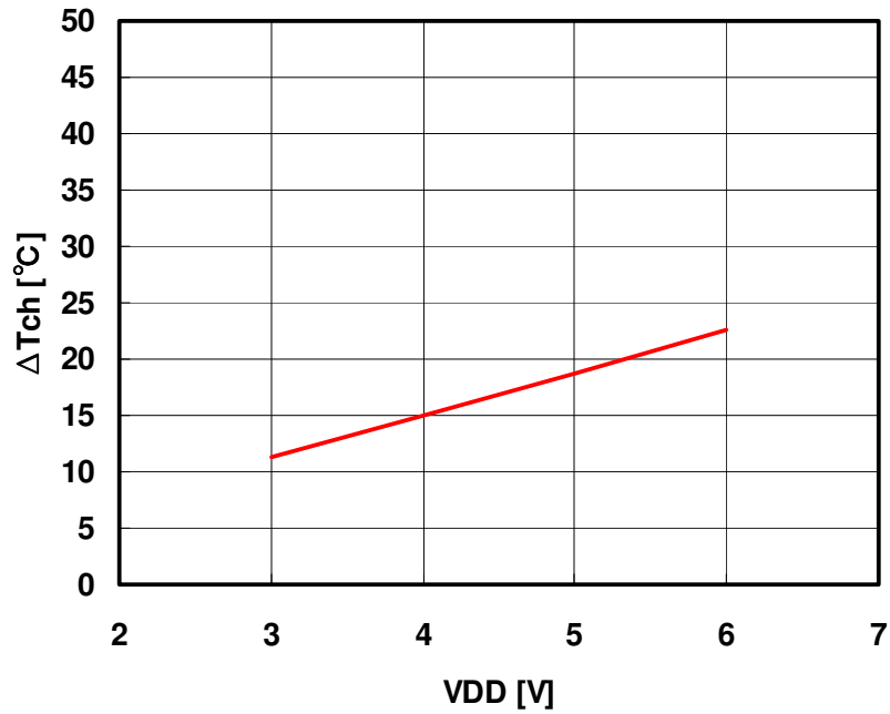
ΔTch vs. Drain Voltage (Reference) IDD=250mA
