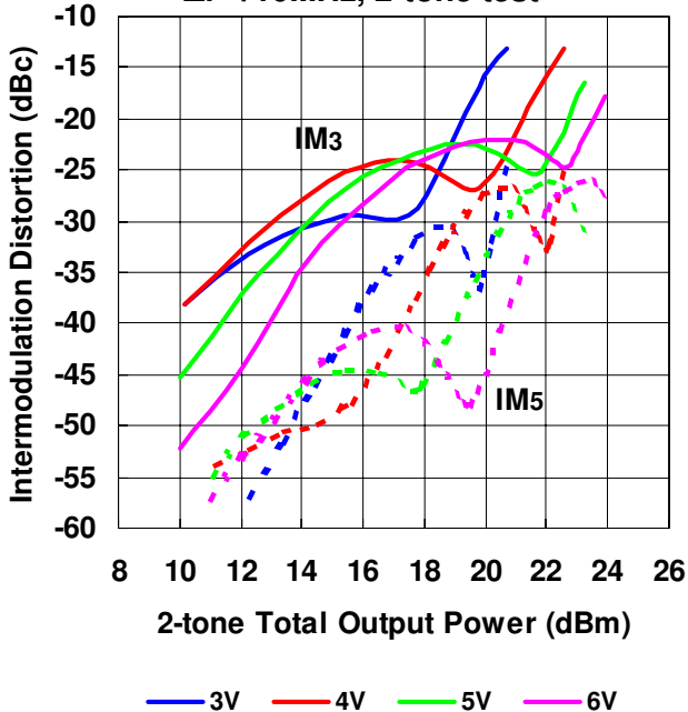
IMD Performance vs. Total Output Power by Drain Voltage
