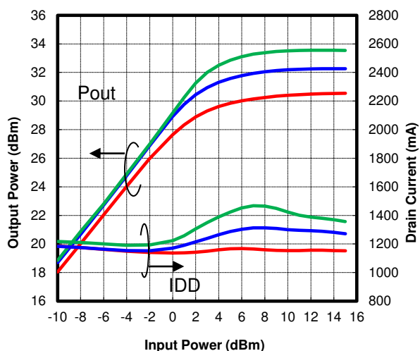
IDD(DC)=1200mA, Freq.=13.5GHz
