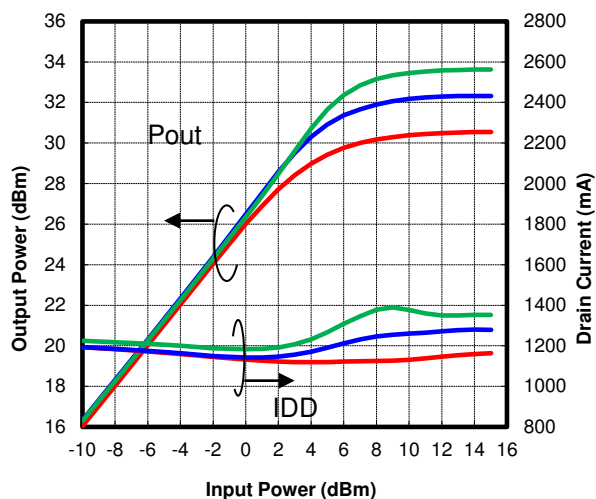
IDD(DC)=1200mA, Freq.=14.5GHz
