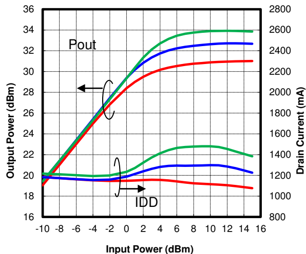
IDD(DC)=1200mA, Freq.=12.7GHz
