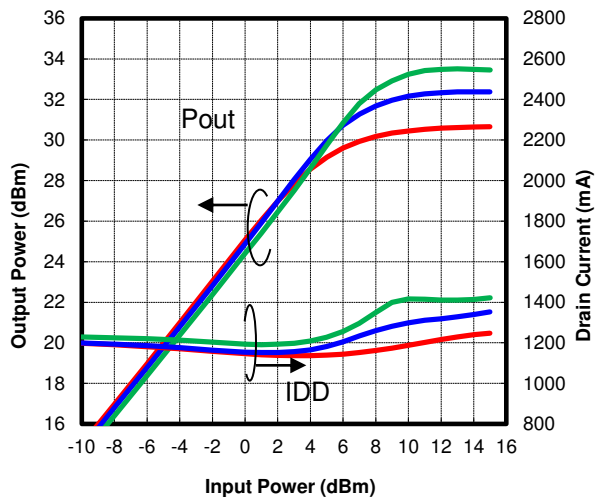
IDD(DC)=1200mA, Freq.=15.4GHz
