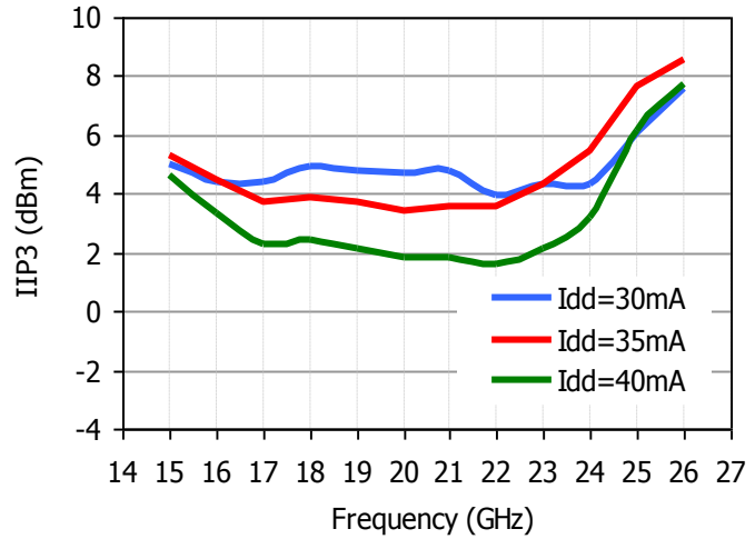
Input IP3 vs. IDD
