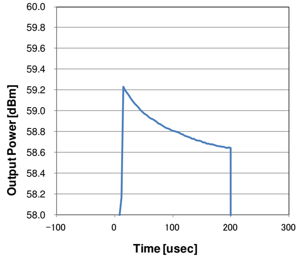
Figure 8. b) f=3.1GHz
