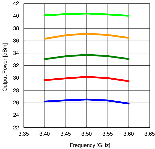
Output Power vs. Frequency V_{DS}=50V I_{DS(DC)}=100mA
