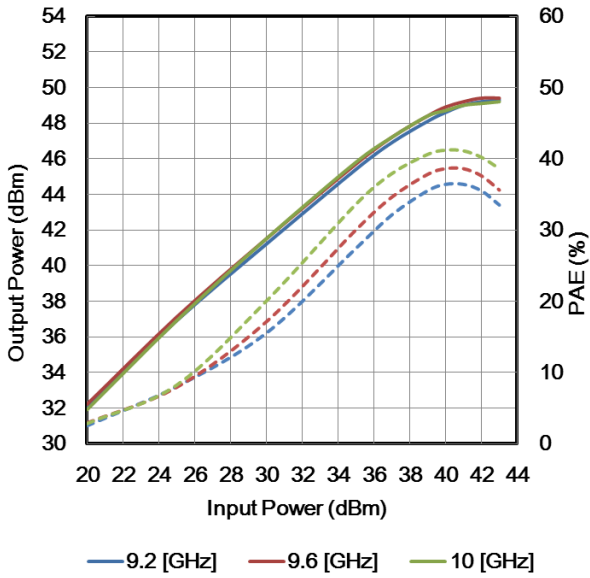
Output Power & Power Added Efficiency vs. Input Power V_{DS}=24V, I_{DS(DC)}=2.6A PW=100usec, Duty 10%
