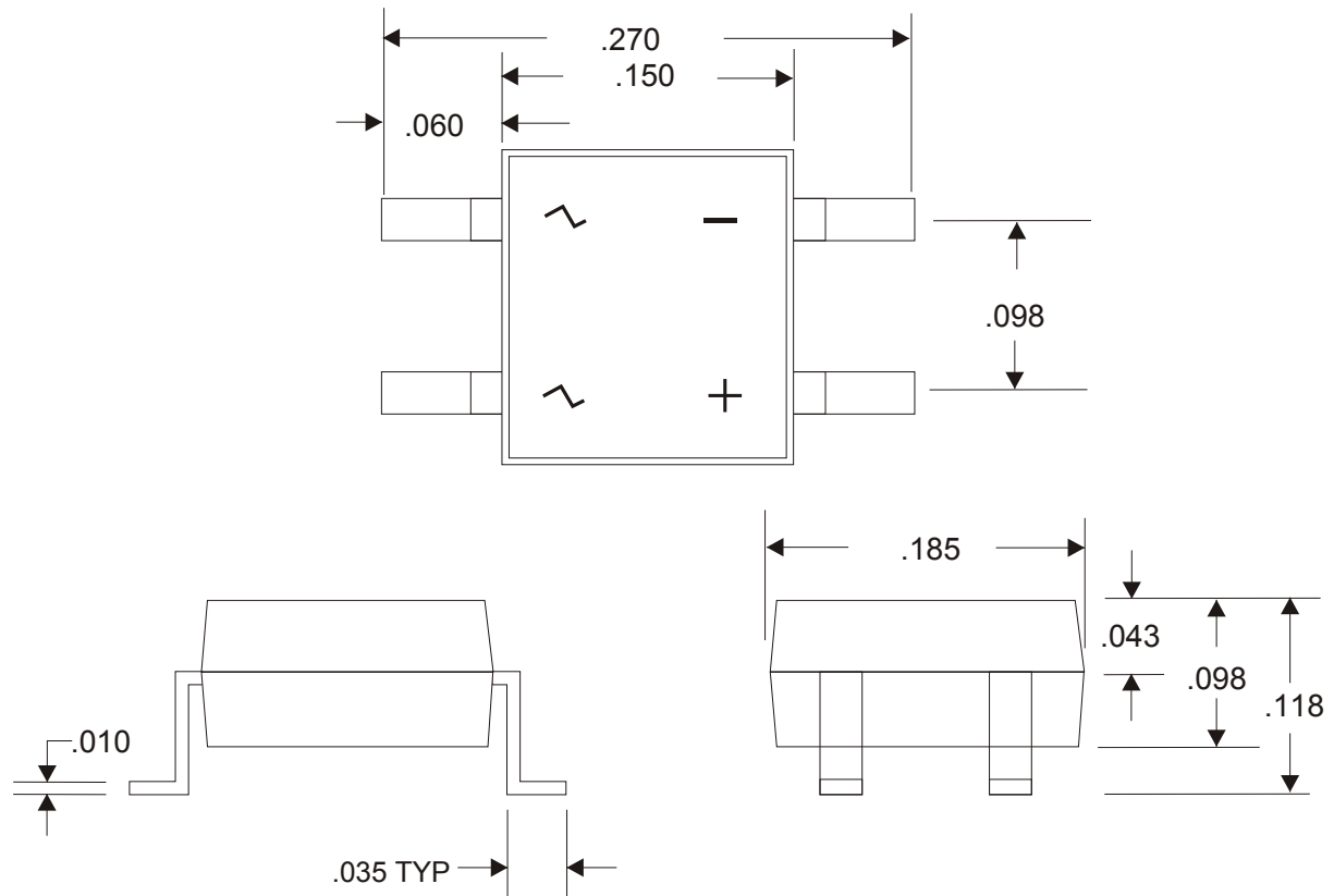
FIG.3 MECHANICAL DIMENSIONS
