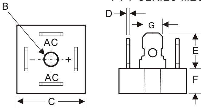
PT-F SERIES MECH. OUTLINE
