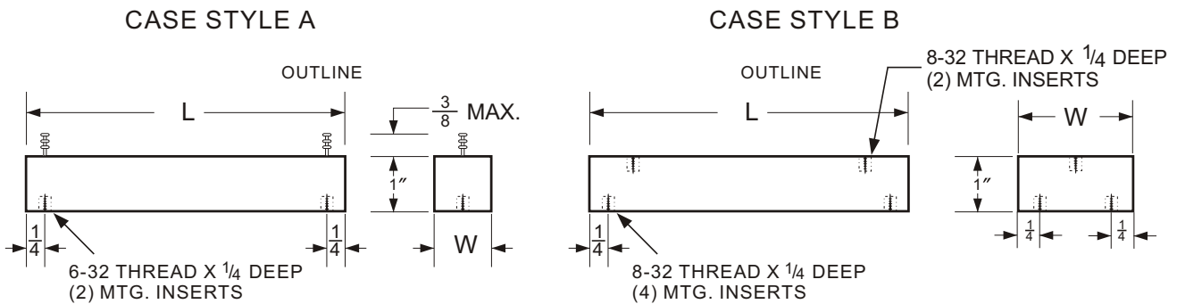
FIG.3 PACKAGE STYLE
