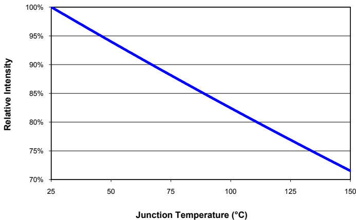
Relative Light Intensity Vs Junction Temperature
