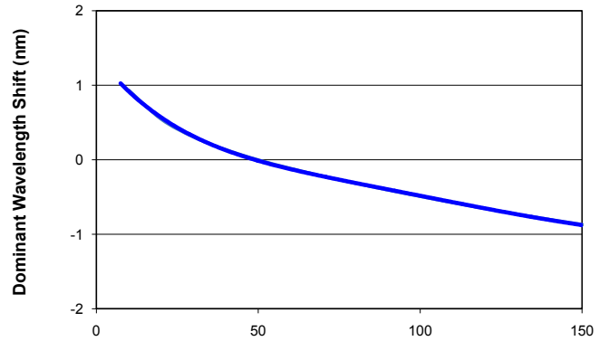
Wavelength Shift vs. Forward Current
