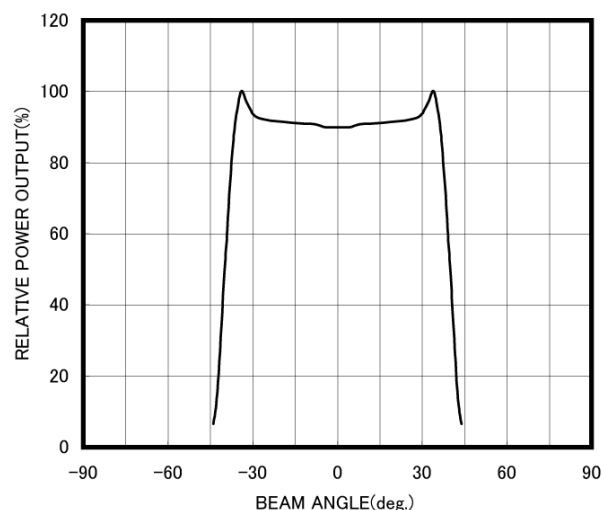
RADIATION PATTERN
