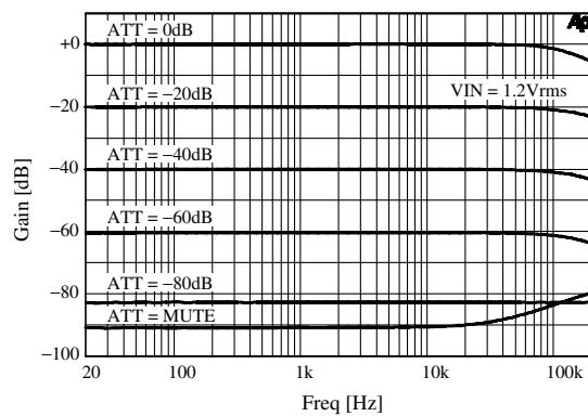
Figure 7. Frequency response
