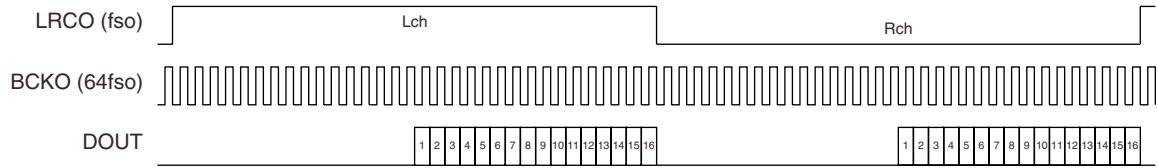
Figure 9. 16-bit MSB-first right-justified (OMOD0 = L, OMOD1 = L, IISO = L), BCKO = 64fso only
